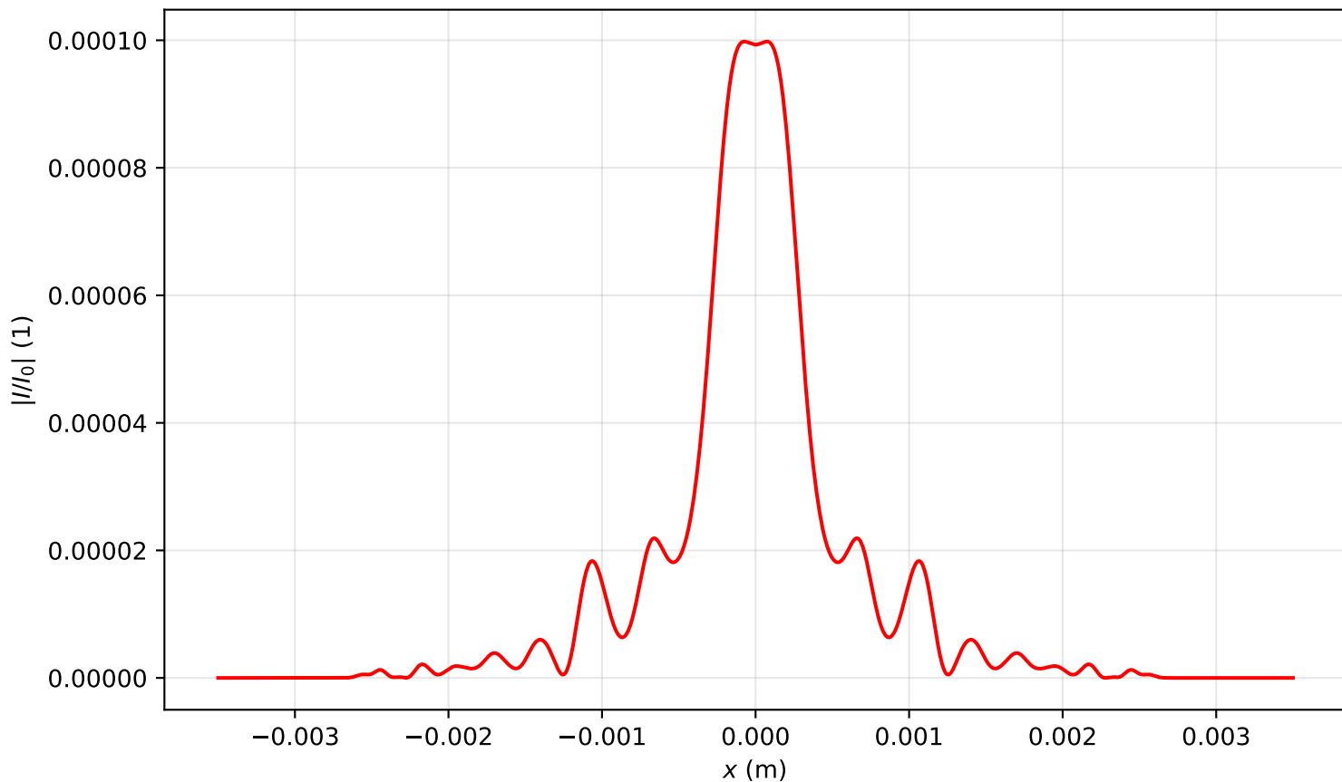
Intensity profile I(x, y = 0, z = 2.149)/I_0 , P_{in}=19.0P_{cr} , artificial time
