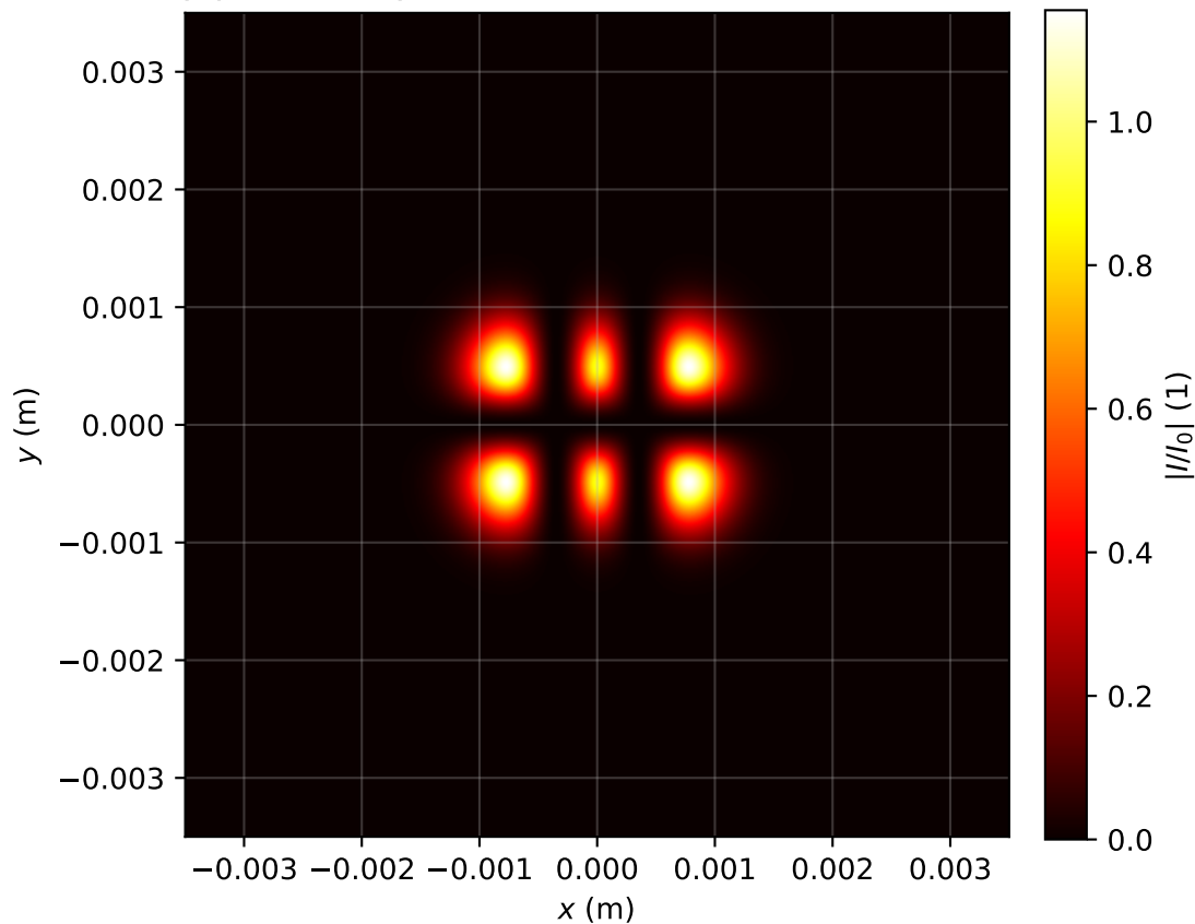
Intensity profile I(x, y, z = 0.080)/I_0 , P_{in}=19.0\text{Pcr} , artificial time
