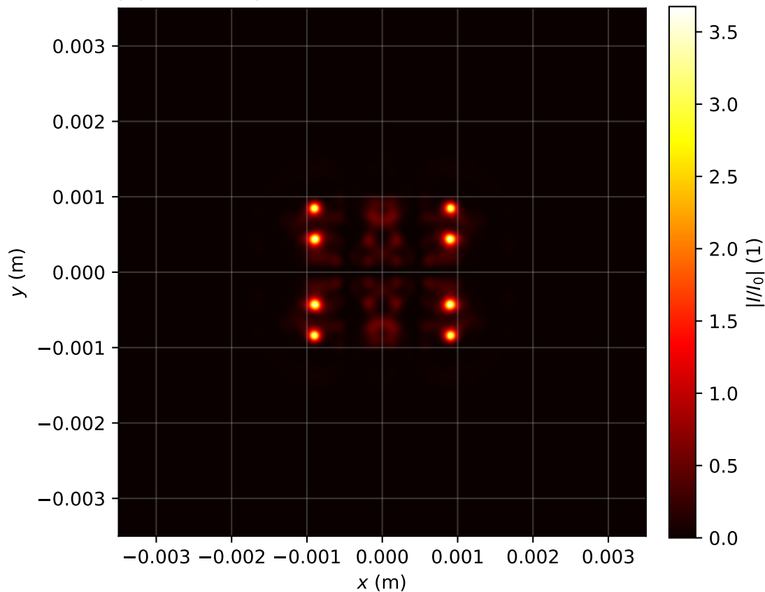
Intensity profile I(x, y, z = 0.796)/I_0 , P_{in}=19.0\text{Pcr} , artificial time
