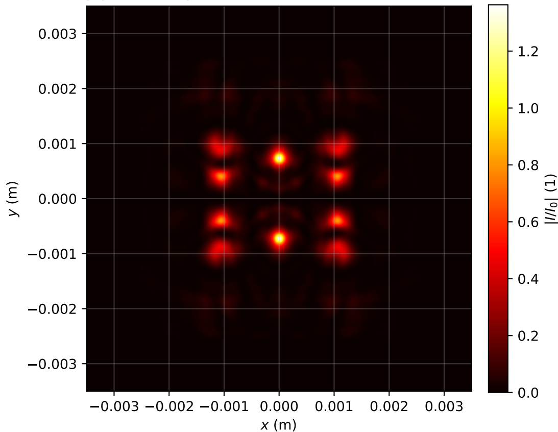
Intensity profile I(x, y, z = 1.751)/I_0 , P_{in}=19.0\text{Pcr} , artificial time
