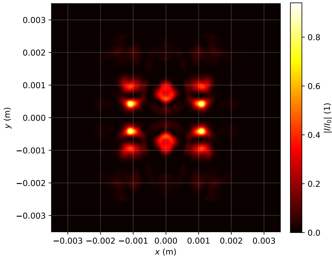
Intensity profile I(x, y, z = 1.831)/I_0 , P_{in}=19.0\text{Pcr} , artificial time
