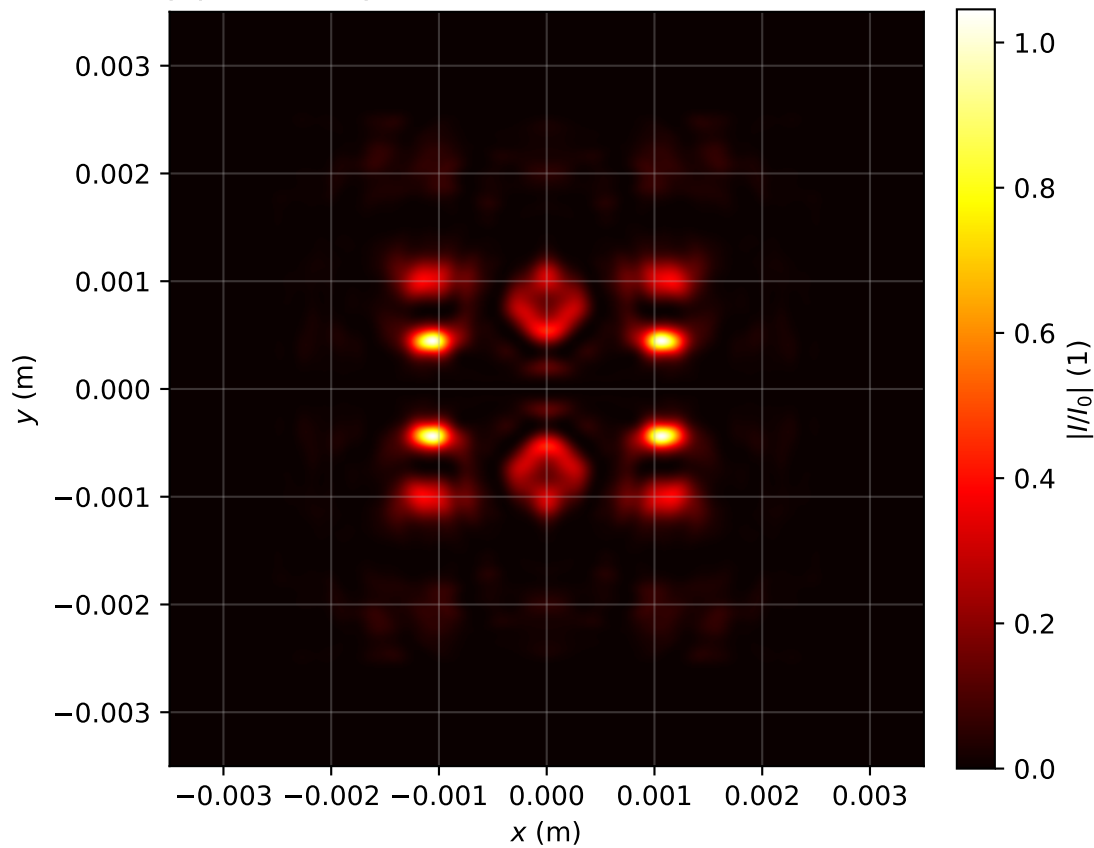
Intensity profile I(x, y, z = 1.911)/I_0 , P_{in}=19.0\text{Pcr} , artificial time
