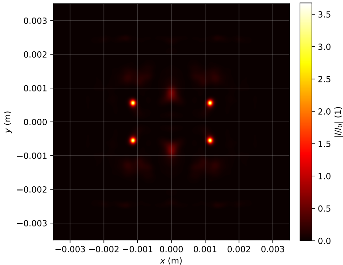
Intensity profile I(x, y, z = 2.388)/I_0 , P_{in}=19.0\text{Pcr} , artificial time
