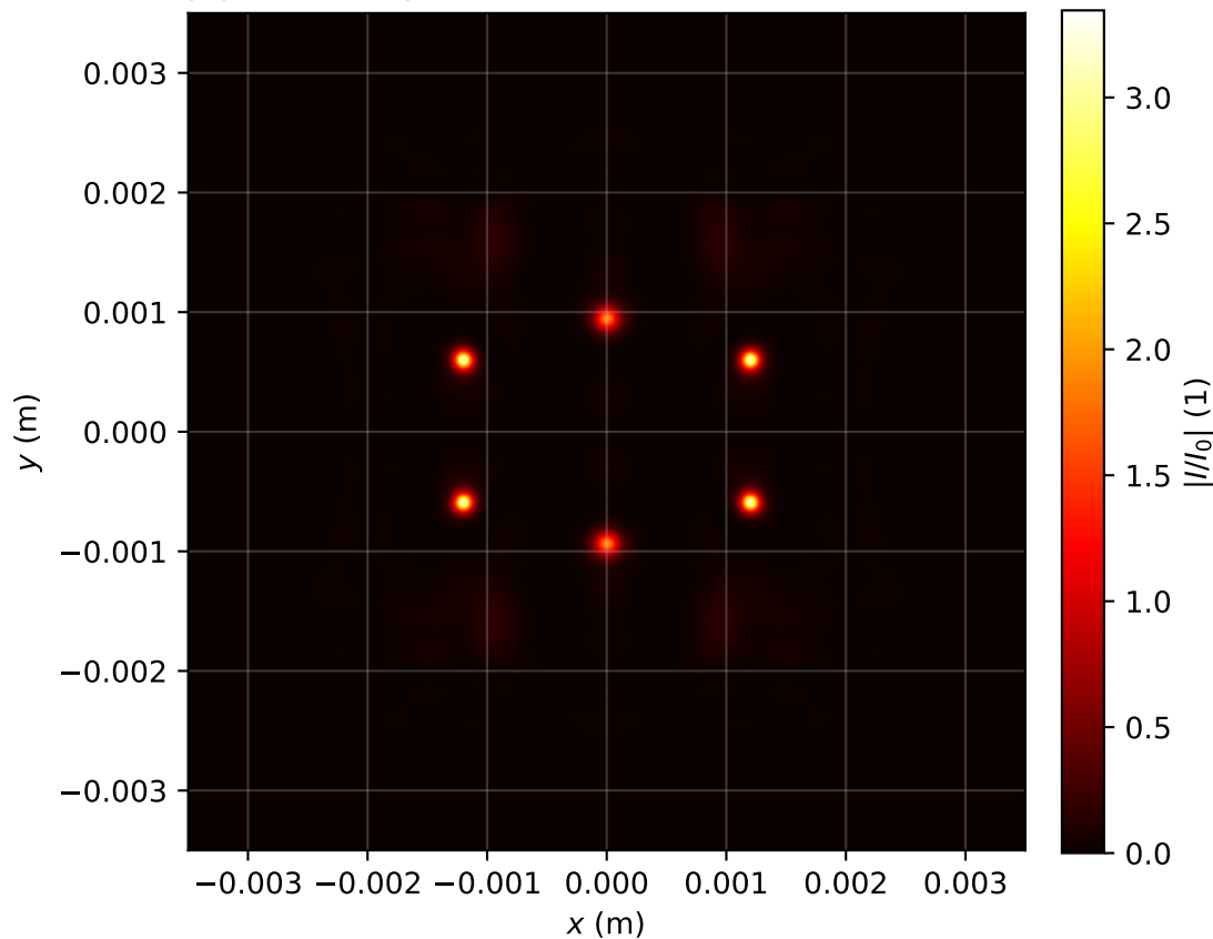
Intensity profile I(x, y, z = 2.707)/I_0 , P_{in}=19.0\text{Pcr} , artificial time
