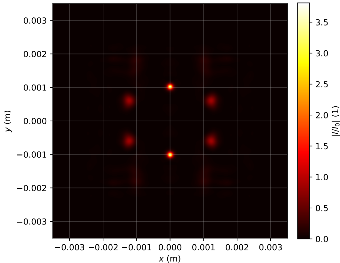
Intensity profile I(x, y, z = 2.866)/I_0 , P_{in}=19.0\text{Pcr} , artificial time
