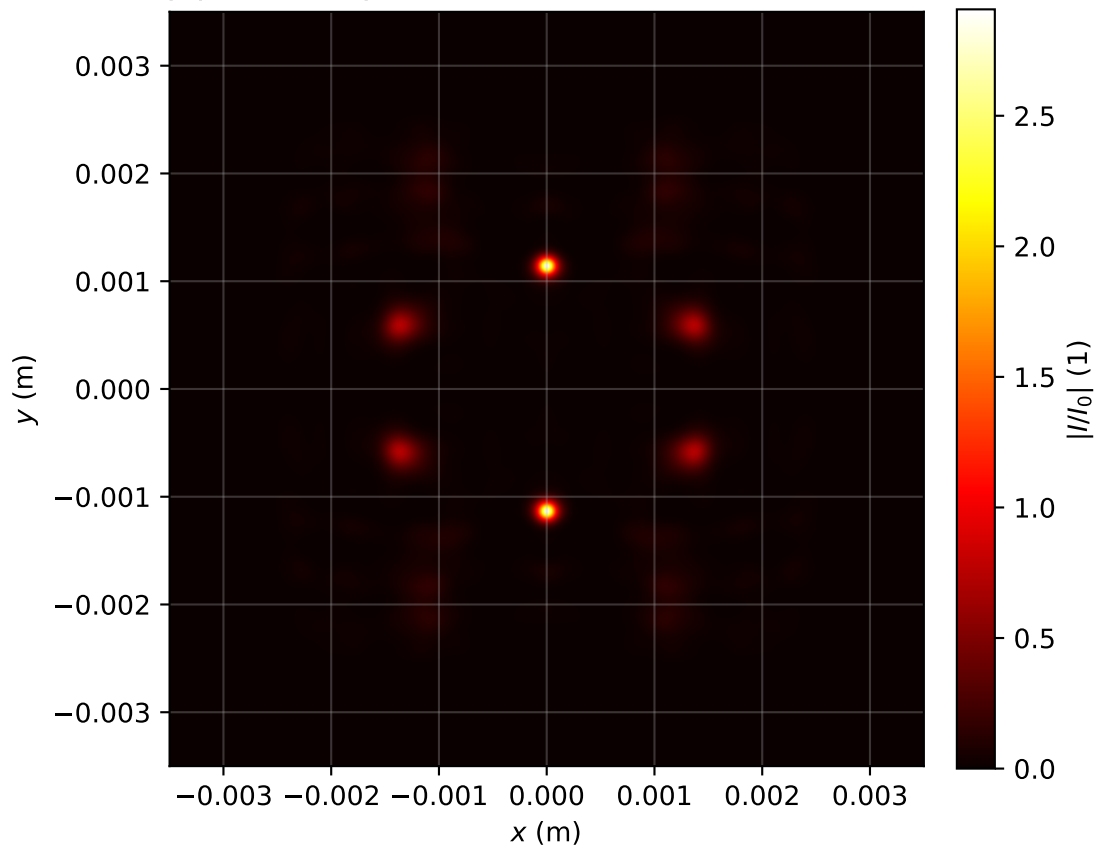
Intensity profile I(x, y, z = 3.184)/I_0 , P_{in}=19.0\text{Pcr} , artificial time
