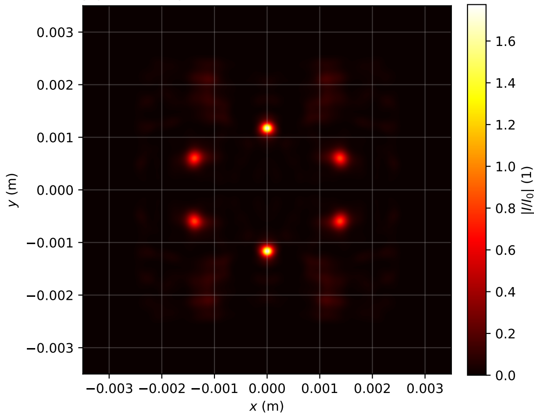
Intensity profile I(x, y, z = 3.264)/I_0 , P_{in}=19.0\text{Pcr} , artificial time
