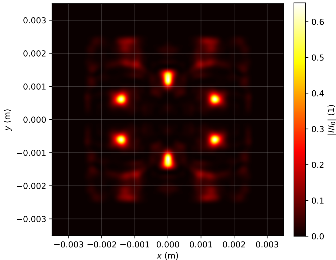
Intensity profile I(x, y, z = 3.423)/I_0 , P_{in}=19.0\text{Pcr} , artificial time
