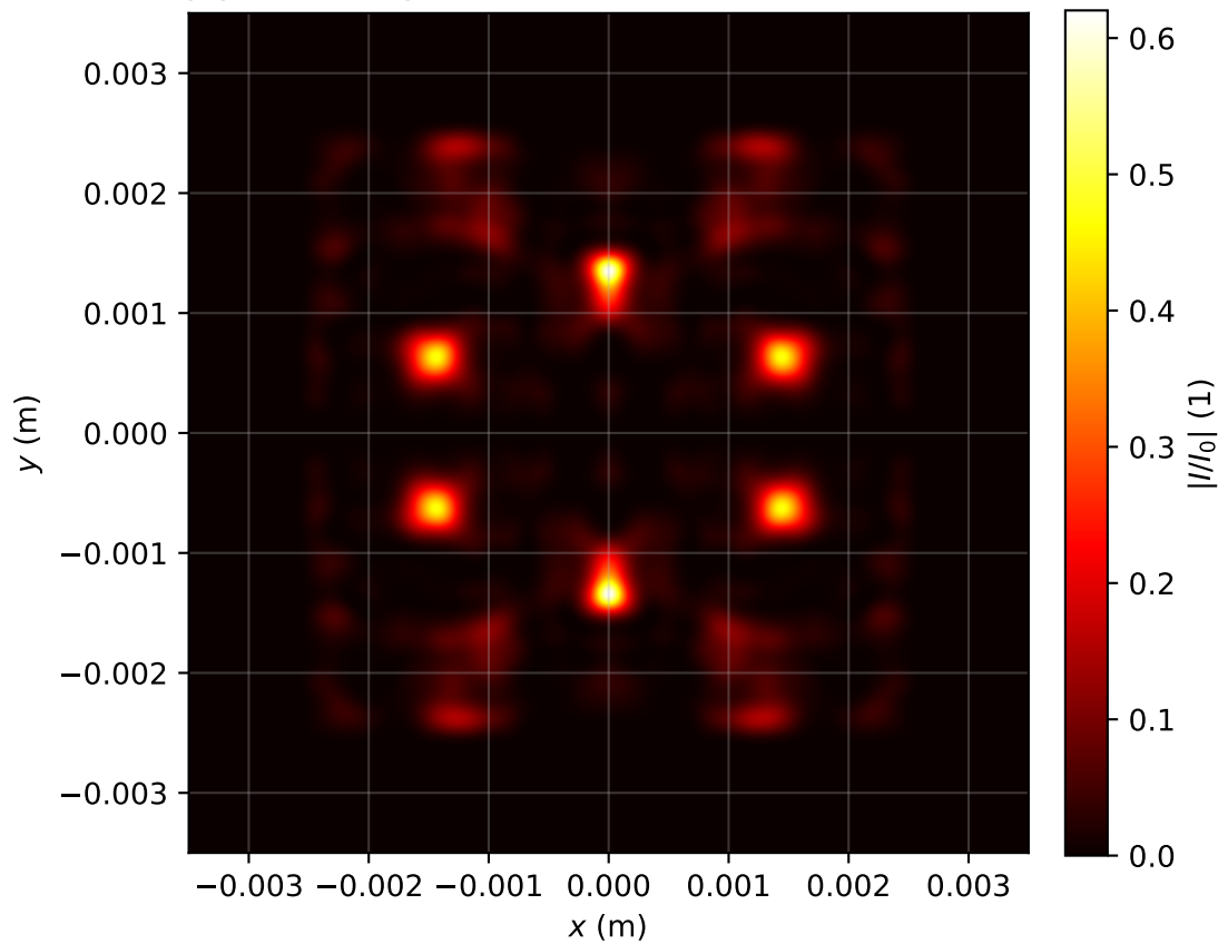
Intensity profile I(x, y, z = 3.503)/I_0 , P_{in}=19.0\text{Pcr} , artificial time
