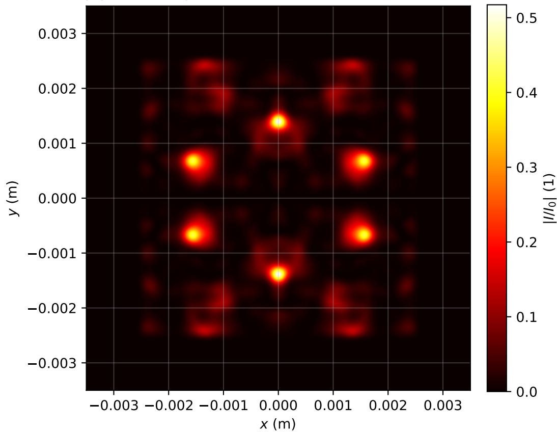
Intensity profile I(x, y, z = 3.662)/I_0 , P_{in}=19.0\text{Pcr} , artificial time
