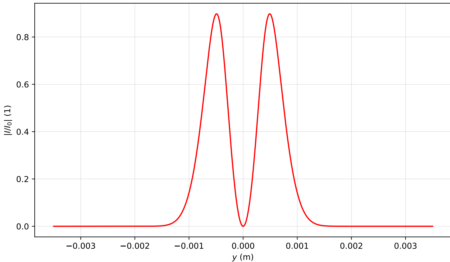
Intensity profile I(x=0, y, z=0.080)/I_0 , P_{in}=19.0P_{cr} , artificial time
