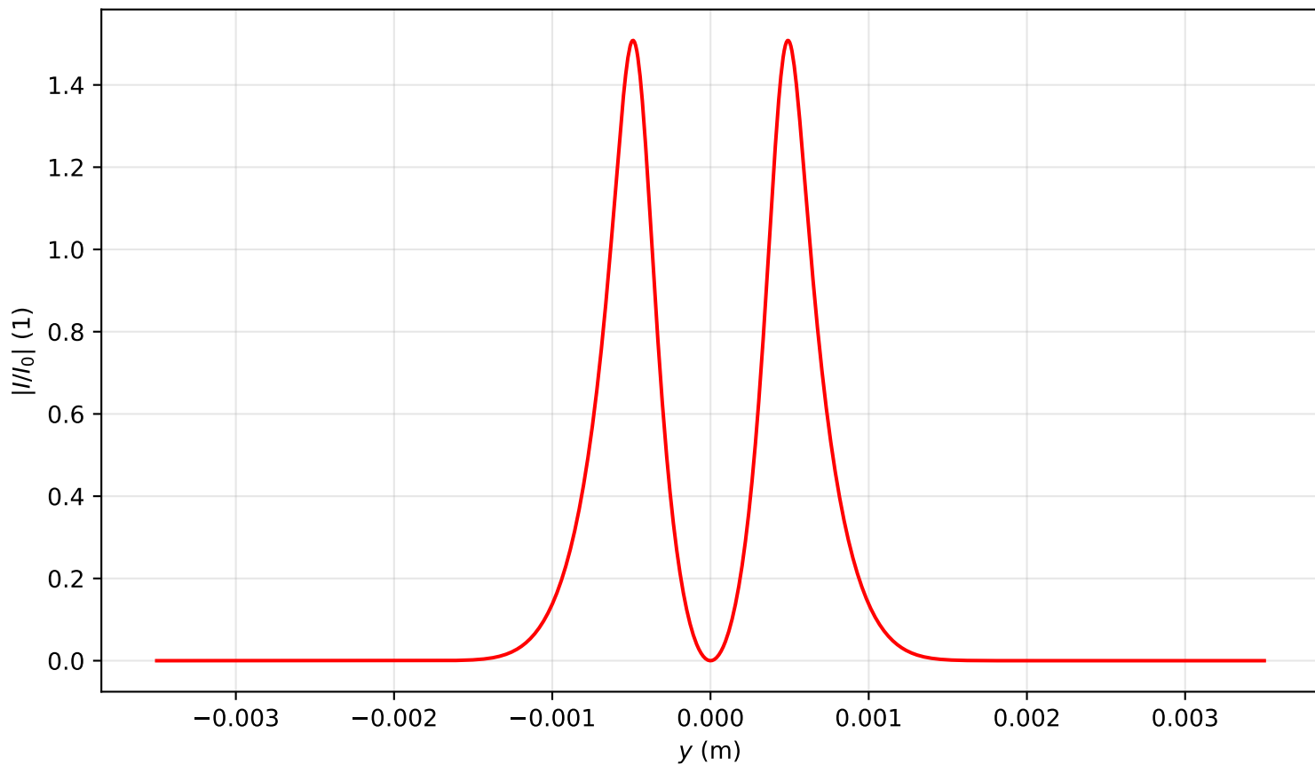
Intensity profile I(x=0, y, z=0.159)/I_0 , P_{in}=19.0P_{cr} , artificial time
