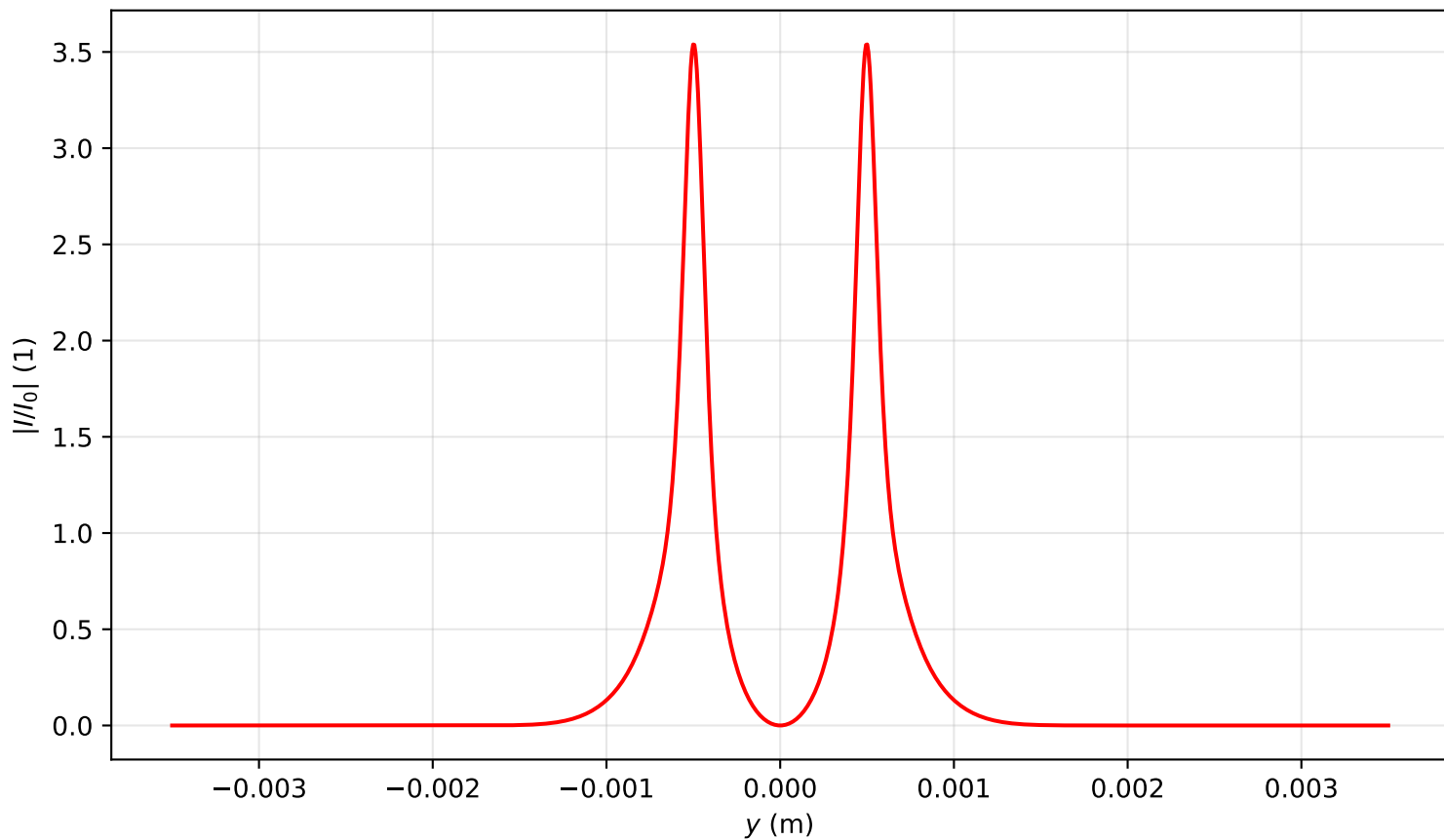
Intensity profile I(x=0, y, z=0.239)/I_0 , P_{in}=19.0P_{cr} , artificial time
