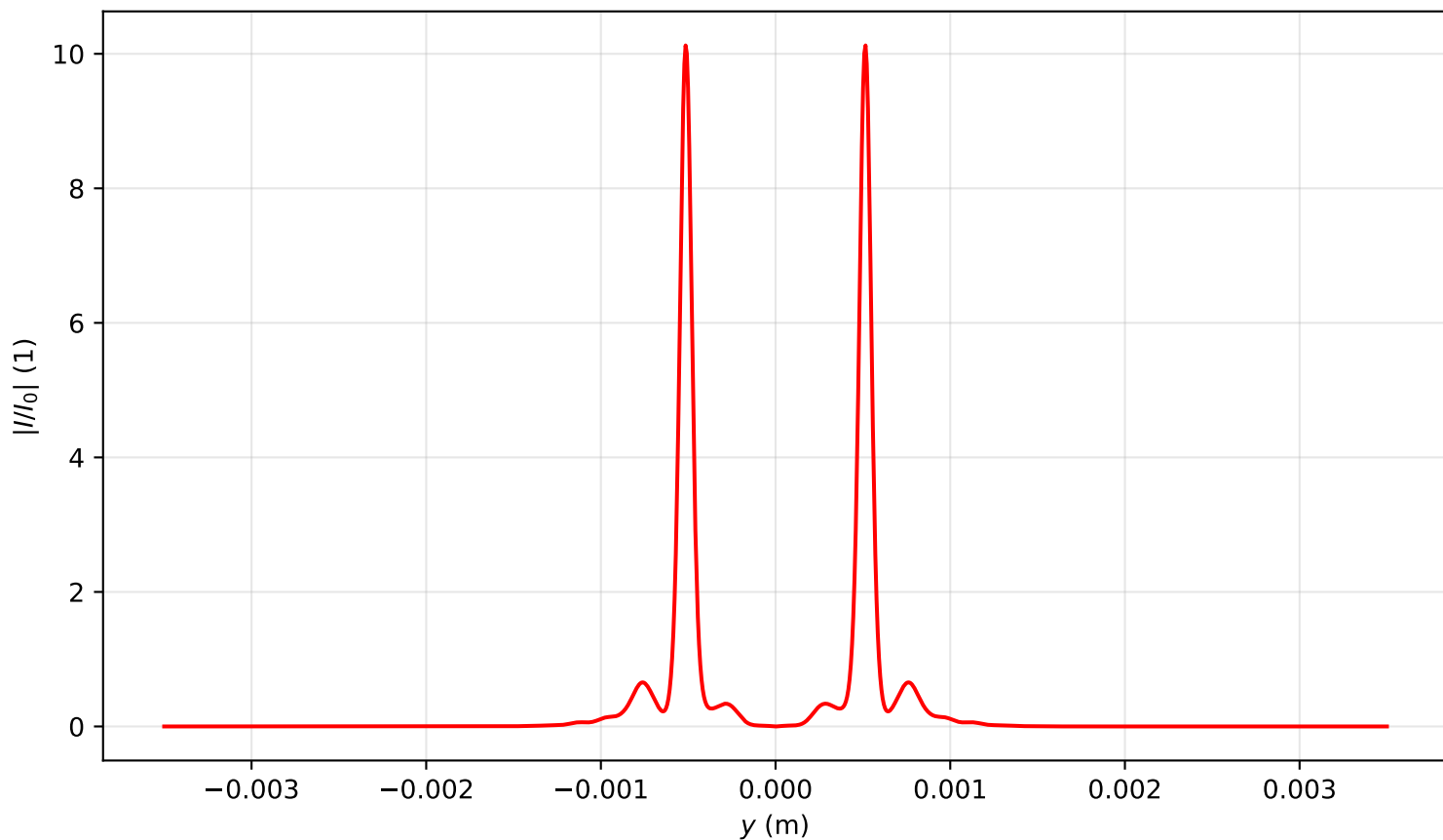
Intensity profile I(x=0, y, z=0.398)/I_0 , Pin=19.0Pcr, artificial time
