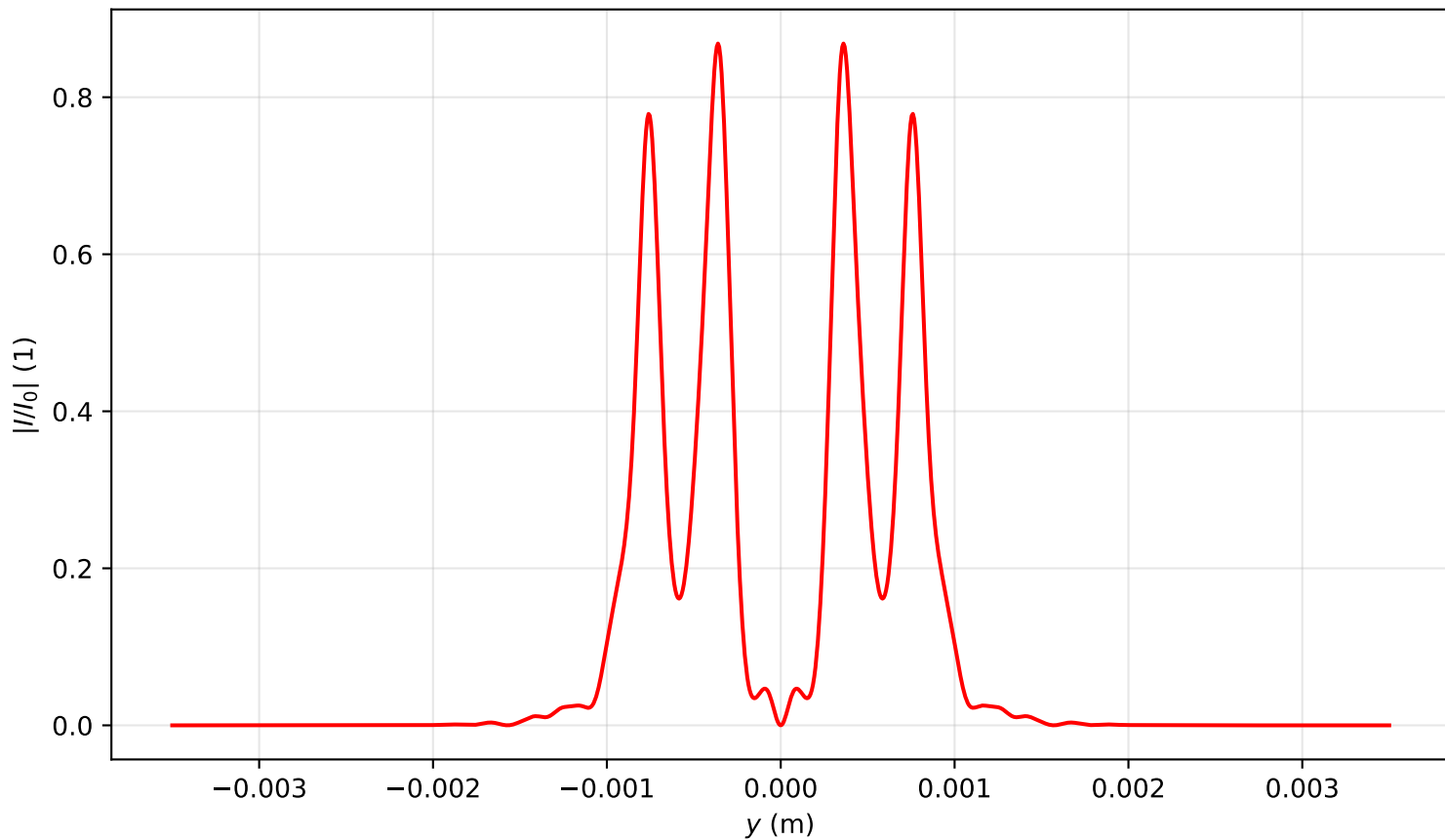
Intensity profile I(x=0, y, z=0.557)/I_0 , P_{in}=19.0\text{Pcr} , artificial time
