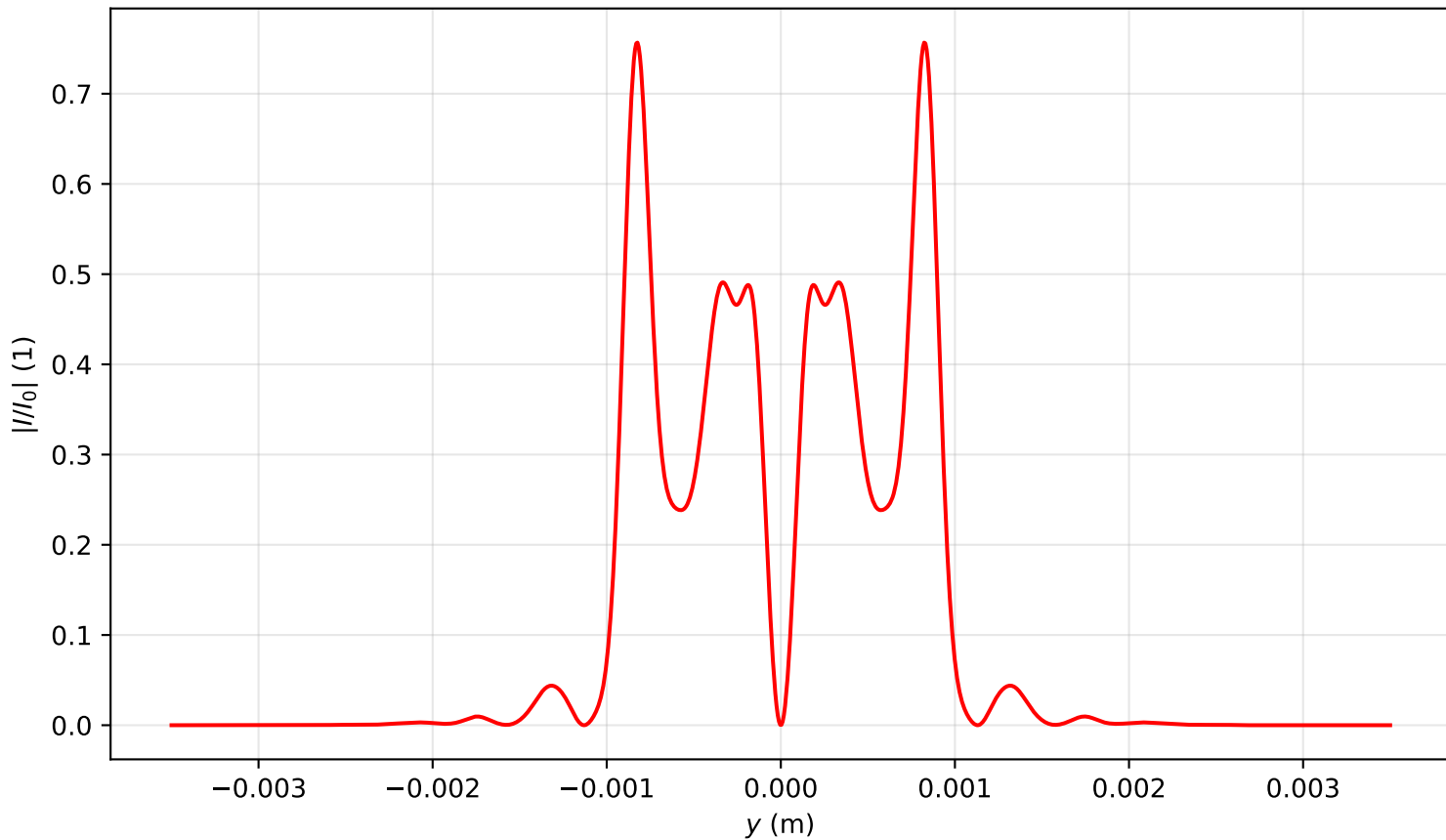
Intensity profile I(x=0, y, z=0.716)/I_0 , P_{in}=19.0\text{Pcr} , artificial time
