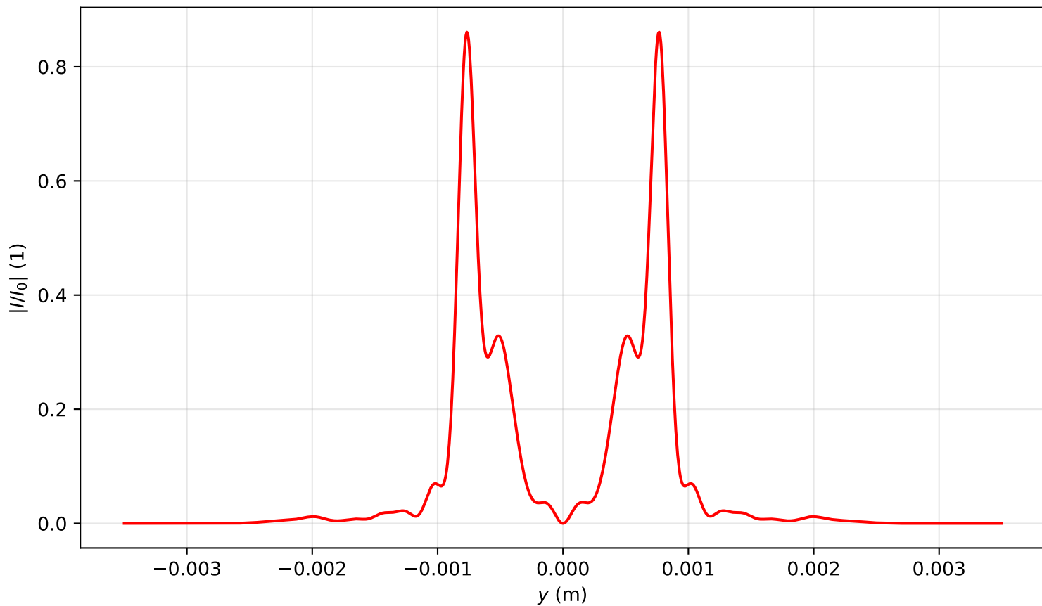
Intensity profile I(x=0, y, z=0.876)/I_0 , P_{in}=19.0\text{Pcr} , artificial time
