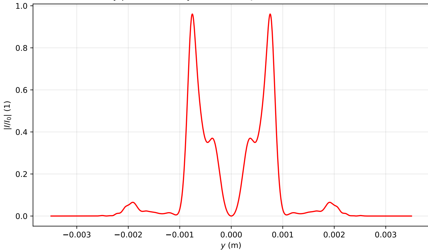
Intensity profile I(x=0, y, z=1.274)/I_0 , P_{in}=19.0\text{Pcr} , artificial time
