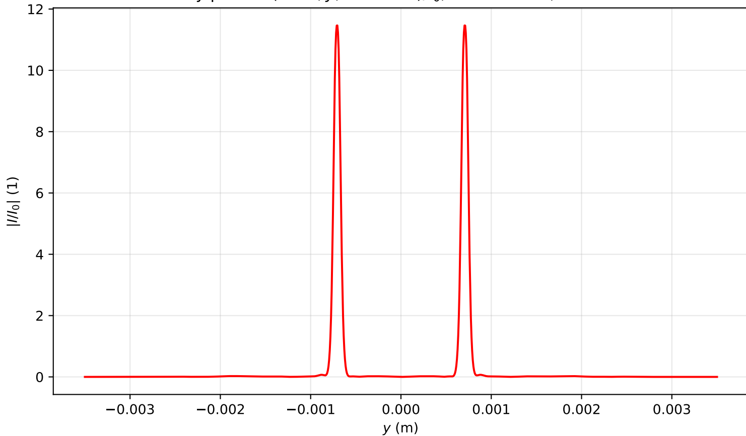
Intensity profile I(x = 0, y, z = 1.592)/I_0 , \text{Pin}=19.0\text{Pcr} , artificial time
