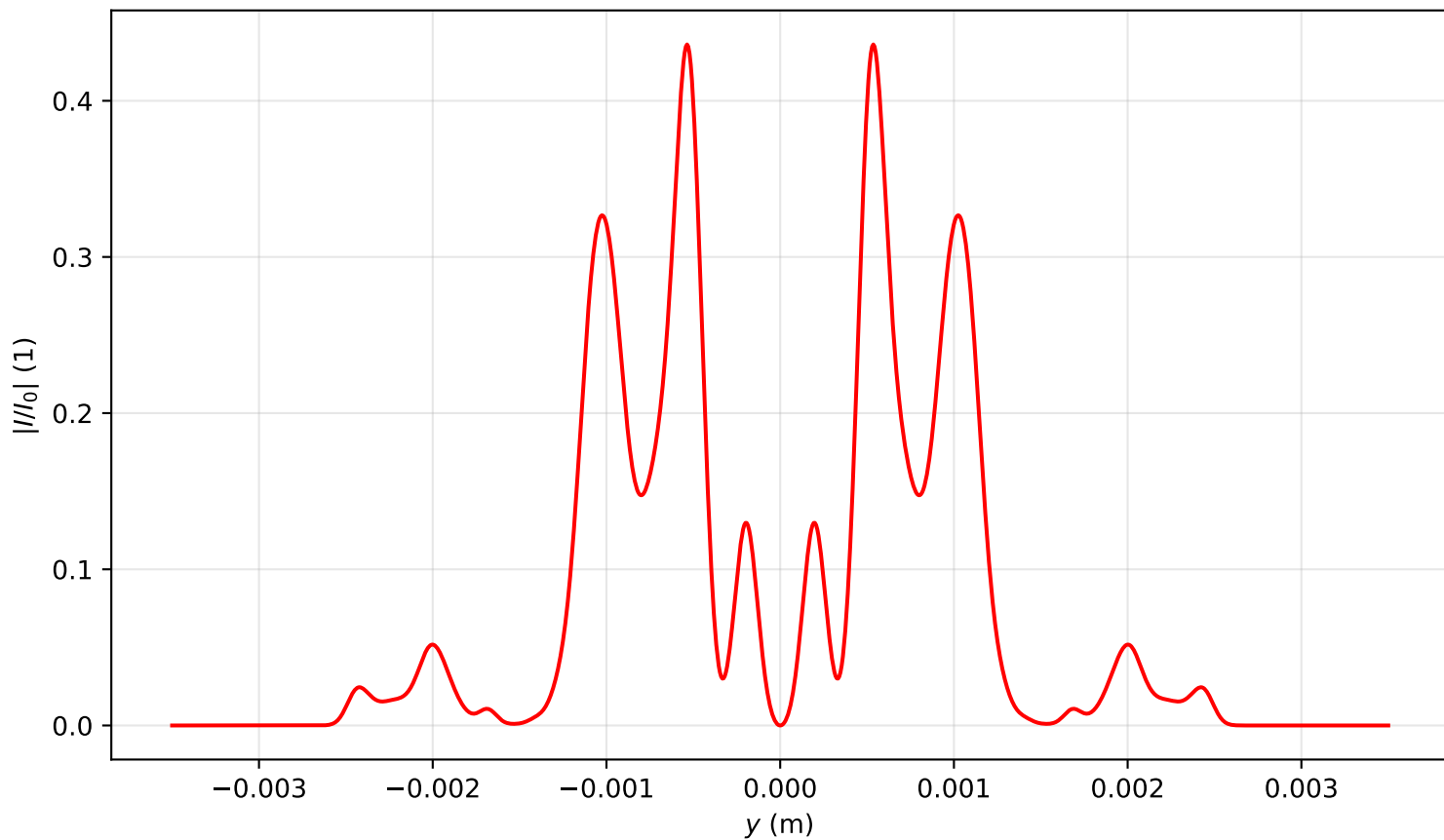
Intensity profile I(x=0, y, z=1.911)/I_0 , P_{in}=19.0\text{Pcr} , artificial time
