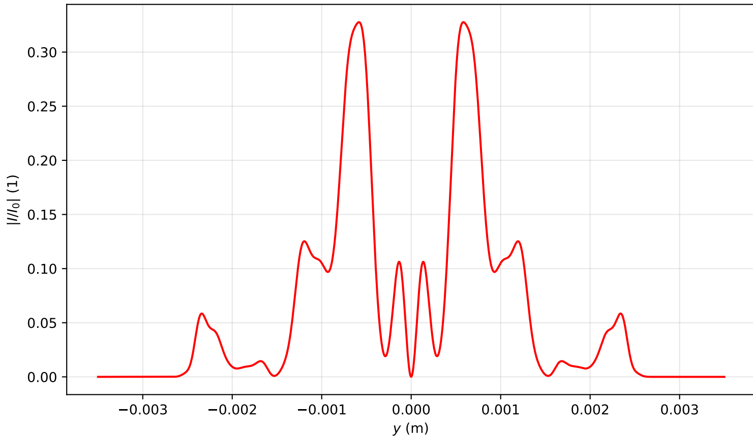
Intensity profile I(x = 0, y, z = 2.070)/I_0 , P_{in}=19.0P_{cr} , artificial time
