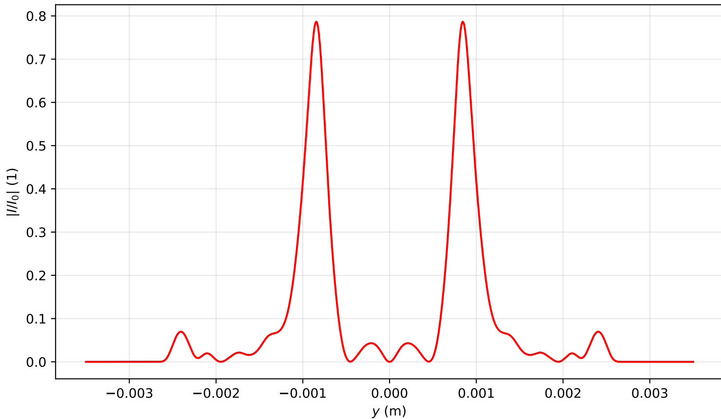
Intensity profile I(x=0, y, z=2.468)/I_0 , P_{in}=19.0P_{cr} , artificial time
