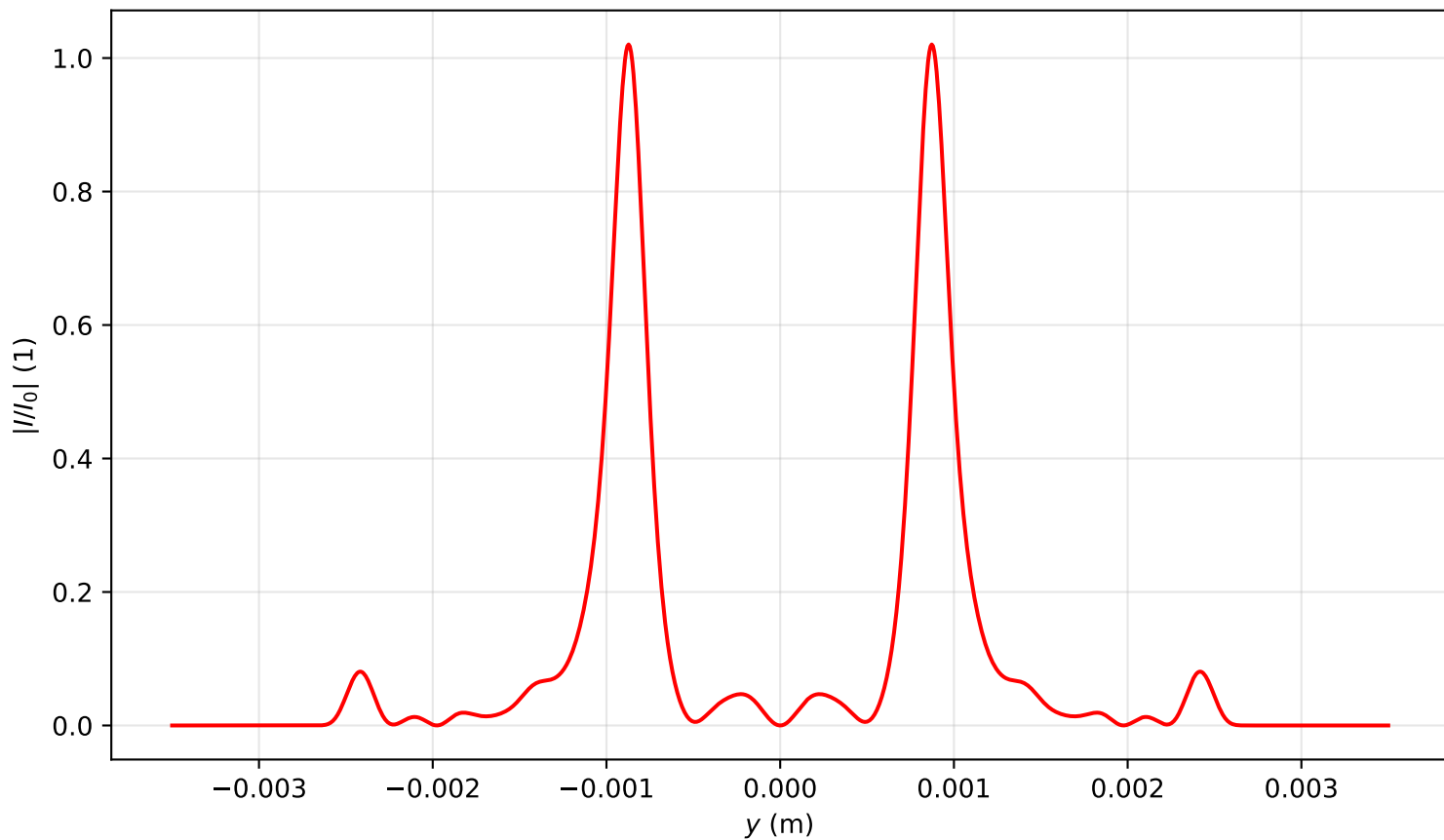
Intensity profile I(x=0, y, z=2.548)/I_0 , P_{in}=19.0P_{cr} , artificial time
