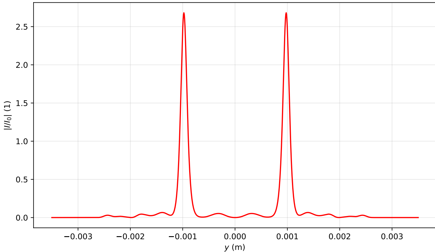
Intensity profile I(x=0, y, z=2.786)/I_0 , P_{in}=19.0\text{Pcr} , artificial time
