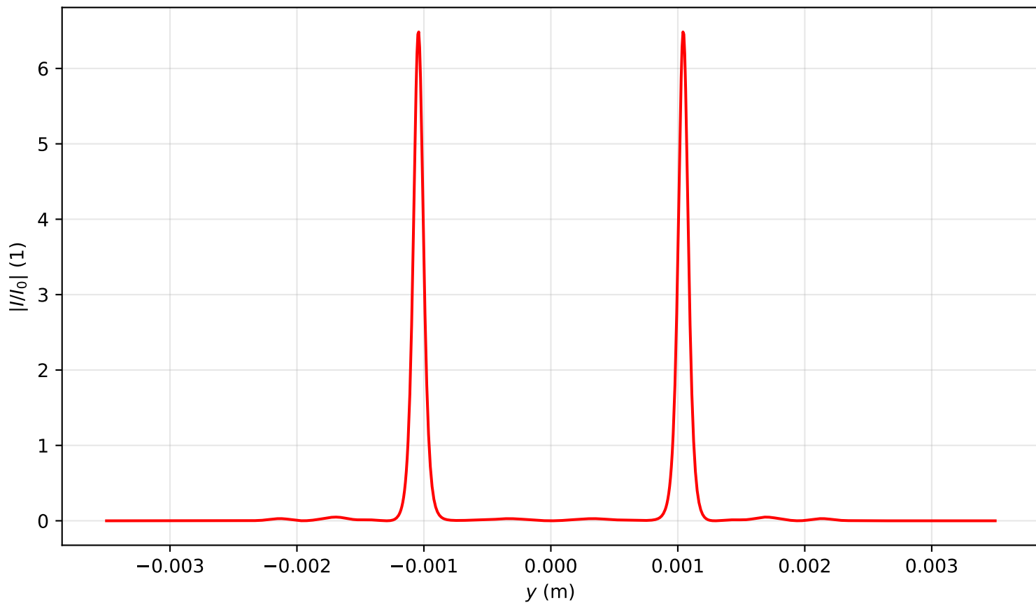
Intensity profile I(x=0, y, z=2.946)/I_0 , P_{in}=19.0\text{Pcr} , artificial time
