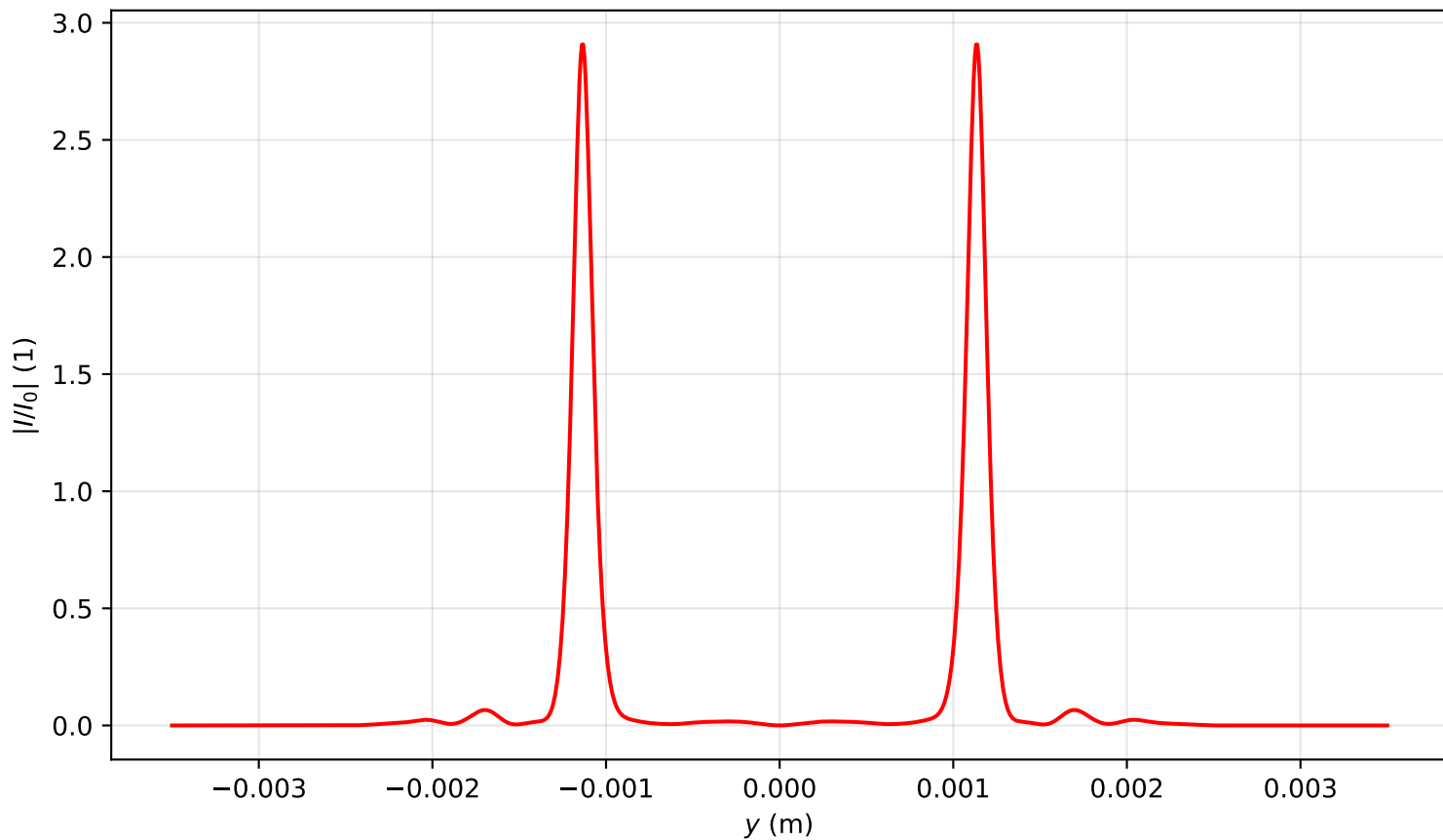
Intensity profile I(x=0, y, z=3.184)/I_0 , P_{in}=19.0P_{cr} , artificial time
