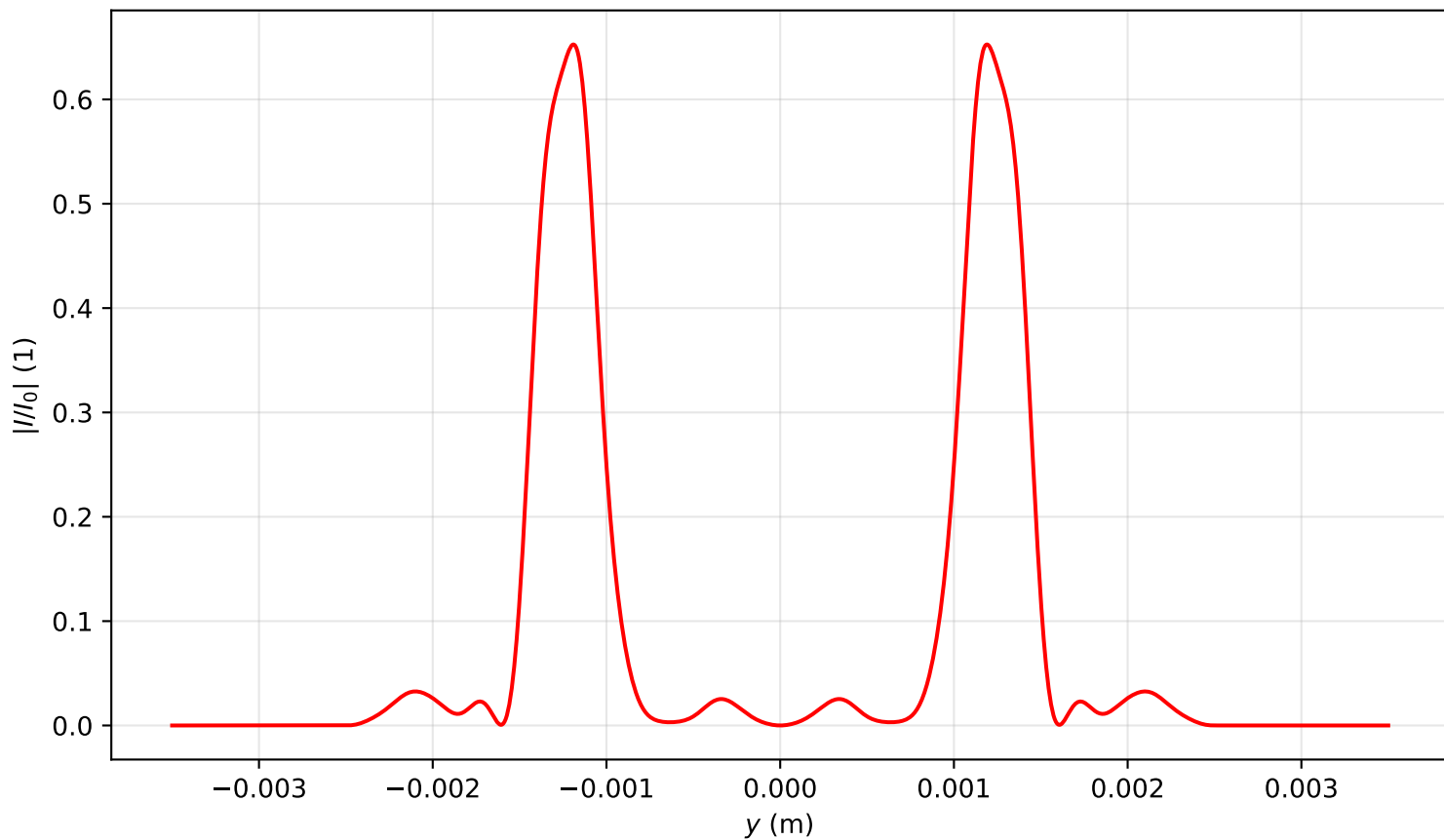
Intensity profile I(x=0, y, z=3.423)/I_0 , P_{in}=19.0\text{Pcr} , artificial time
