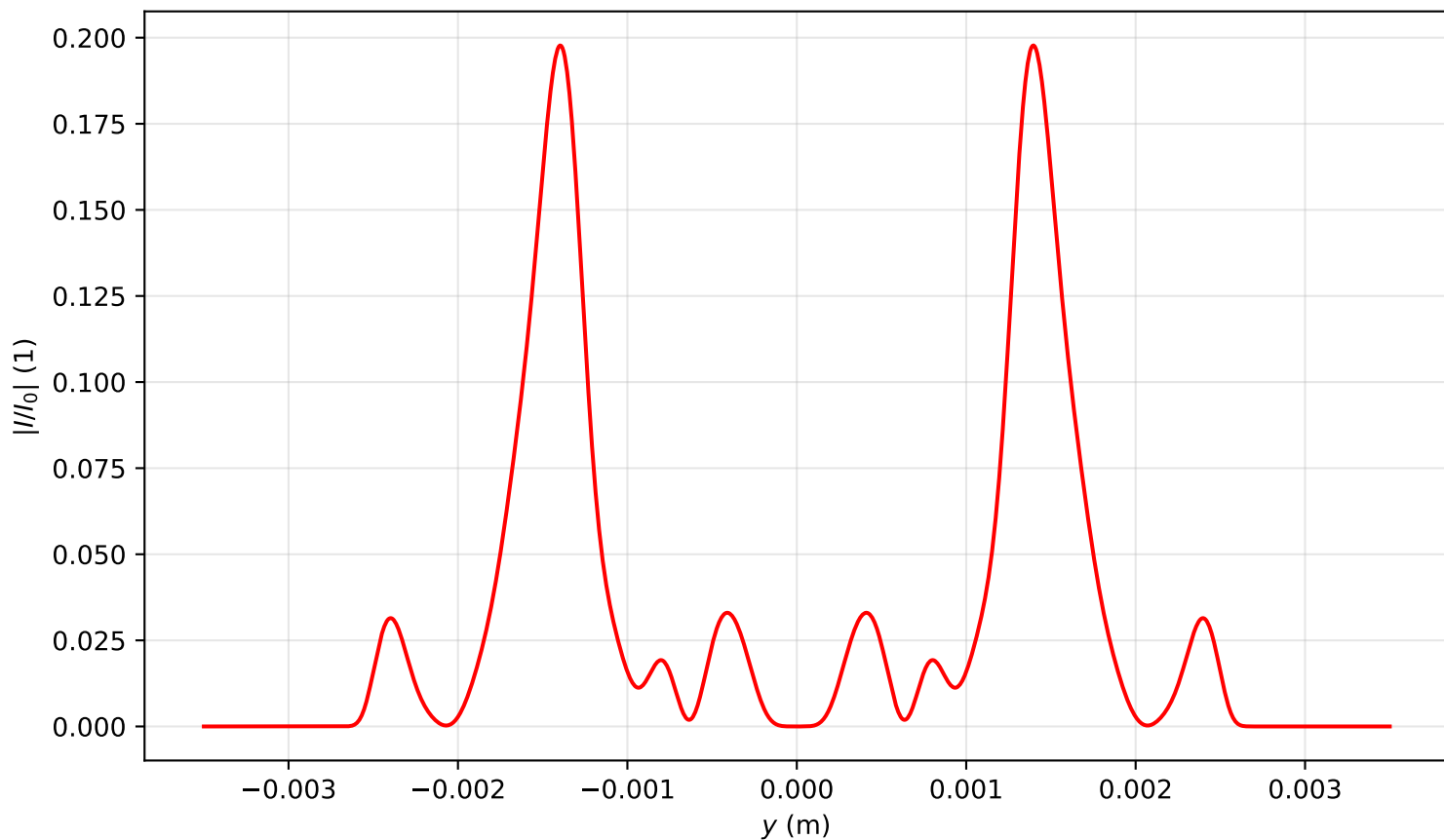
Intensity profile I(x=0, y, z=3.901)/I_0 , P_{in}=19.0P_{cr} , artificial time
