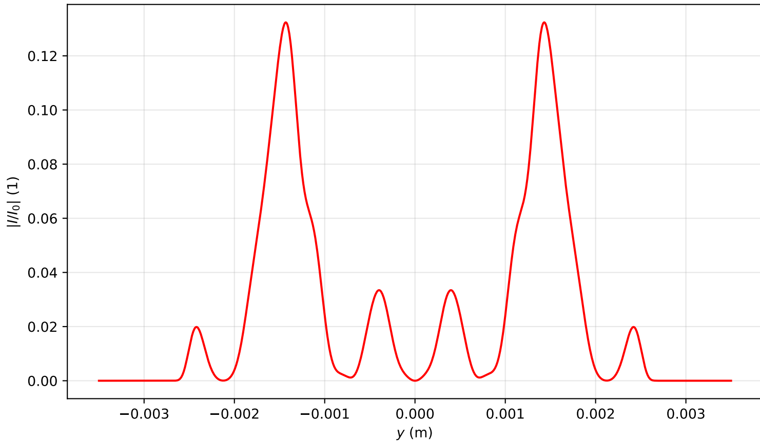
Intensity profile I(x = 0, y, z = 3.981)/I_0 , P_{in}=19.0\text{Pcr} , artificial time
