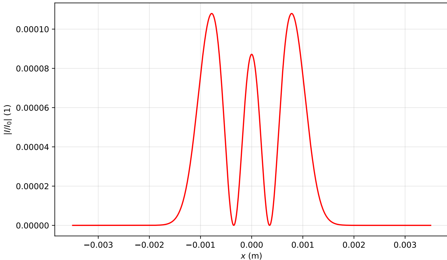
Intensity profile I(x, y = 0, z = 0.080)/I_0 , P_{in}=20.0P_{cr} , artificial time
