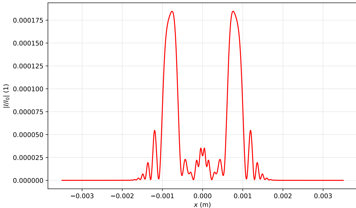
Intensity profile I(x, y = 0, z = 0.318)/I_0 , P_{in}=20.0\text{Pcr} , artificial time
