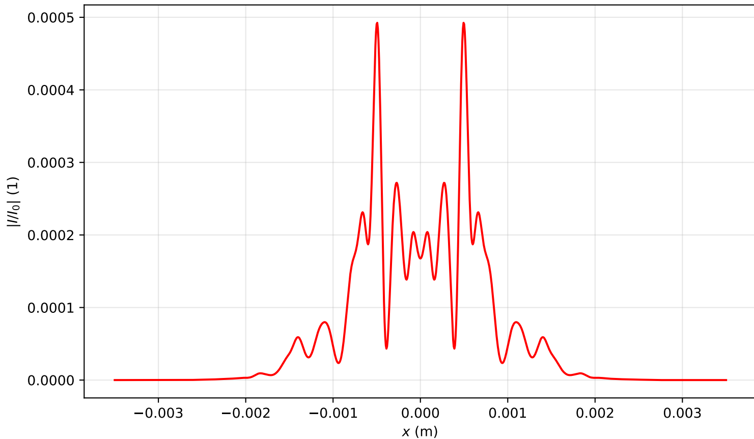
Intensity profile I(x, y = 0, z = 0.557)/I_0 , P_{in}=20.0\text{Pcr} , artificial time
