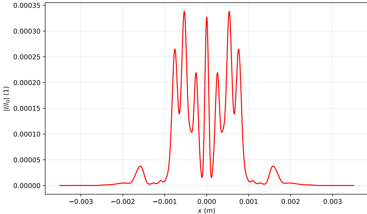
Intensity profile I(x, y = 0, z = 0.637)/I_0 , P_{in}=20.0P_{cr} , artificial time
