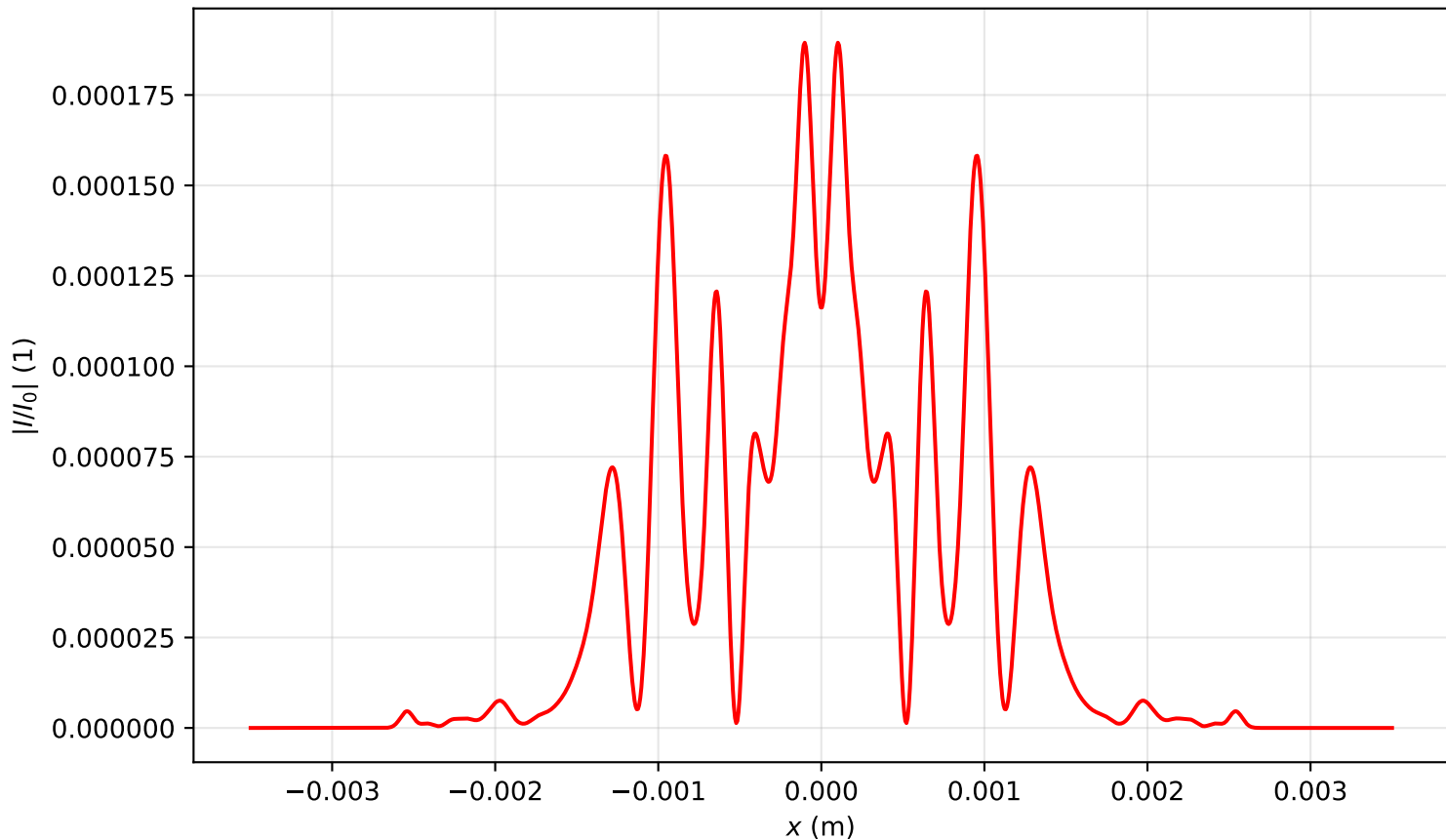
Intensity profile I(x, y = 0, z = 1.035)/I_0 , P_{in}=20.0\text{Pcr} , artificial time
