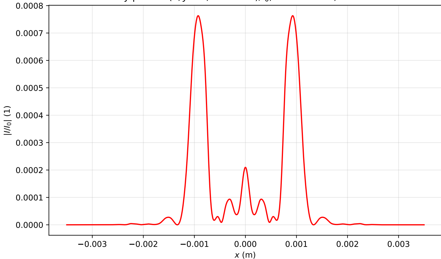
Intensity profile I(x, y = 0, z = 1.115)/I_0 , P_{in}=20.0\text{Pcr} , artificial time
