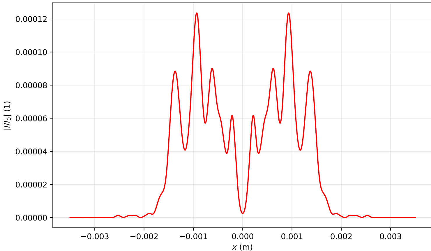
Intensity profile I(x, y = 0, z = 1.433)/I_0 , P_{in}=20.0P_{cr} , artificial time
