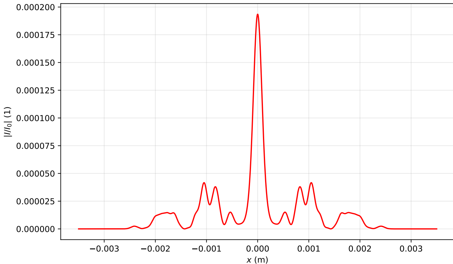
Intensity profile I(x, y = 0, z = 1.751)/I_0 , P_{in}=20.0\text{Pcr} , artificial time
