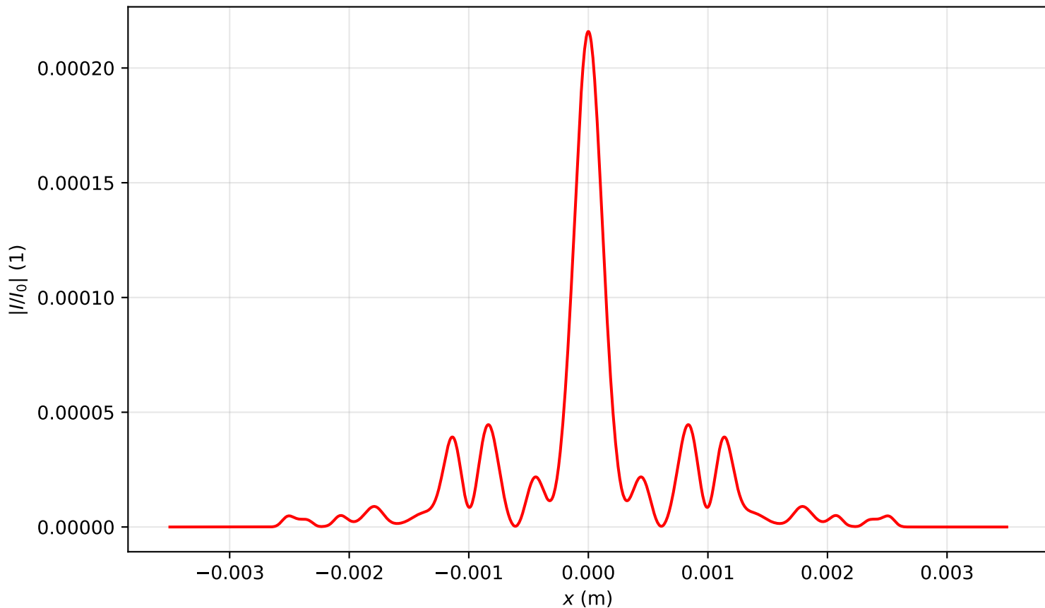
Intensity profile I(x, y = 0, z = 1.990)/I_0 , P_{in}=20.0P_{cr} , artificial time
