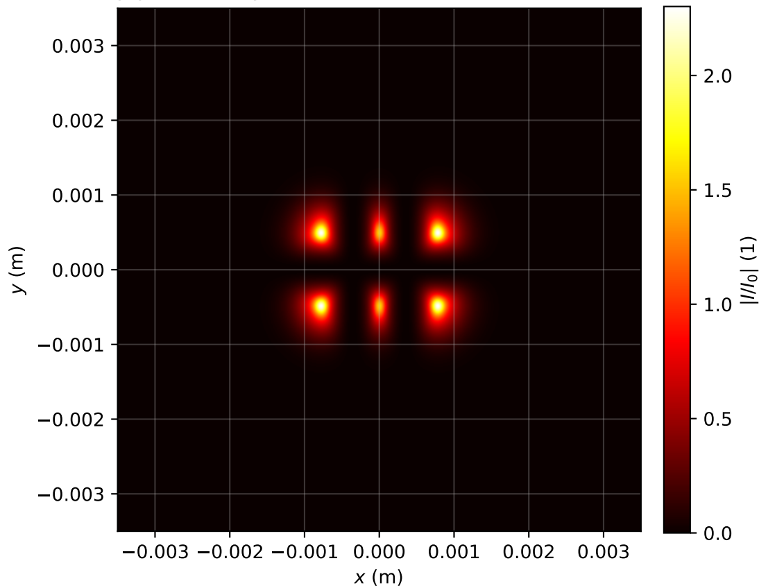
Intensity profile I(x, y, z = 0.159)/I_0 , P_{in}=20.0\text{Pcr} , artificial time
