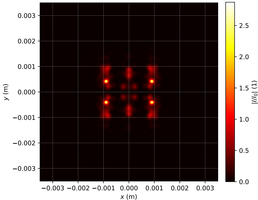
Intensity profile I(x, y, z = 0.955)/I_0 , P_{in}=20.0\text{Pcr} , artificial time
