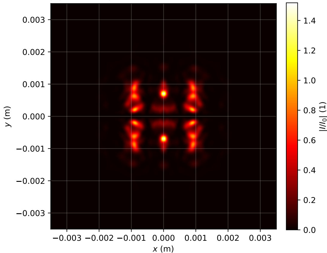
Intensity profile I(x, y, z = 1.035)/I_0 , P_{in}=20.0\text{Pcr} , artificial time
