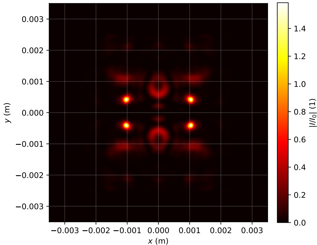
Intensity profile I(x, y, z = 1.911)/I_0 , P_{in}=20.0\text{Pcr} , artificial time
