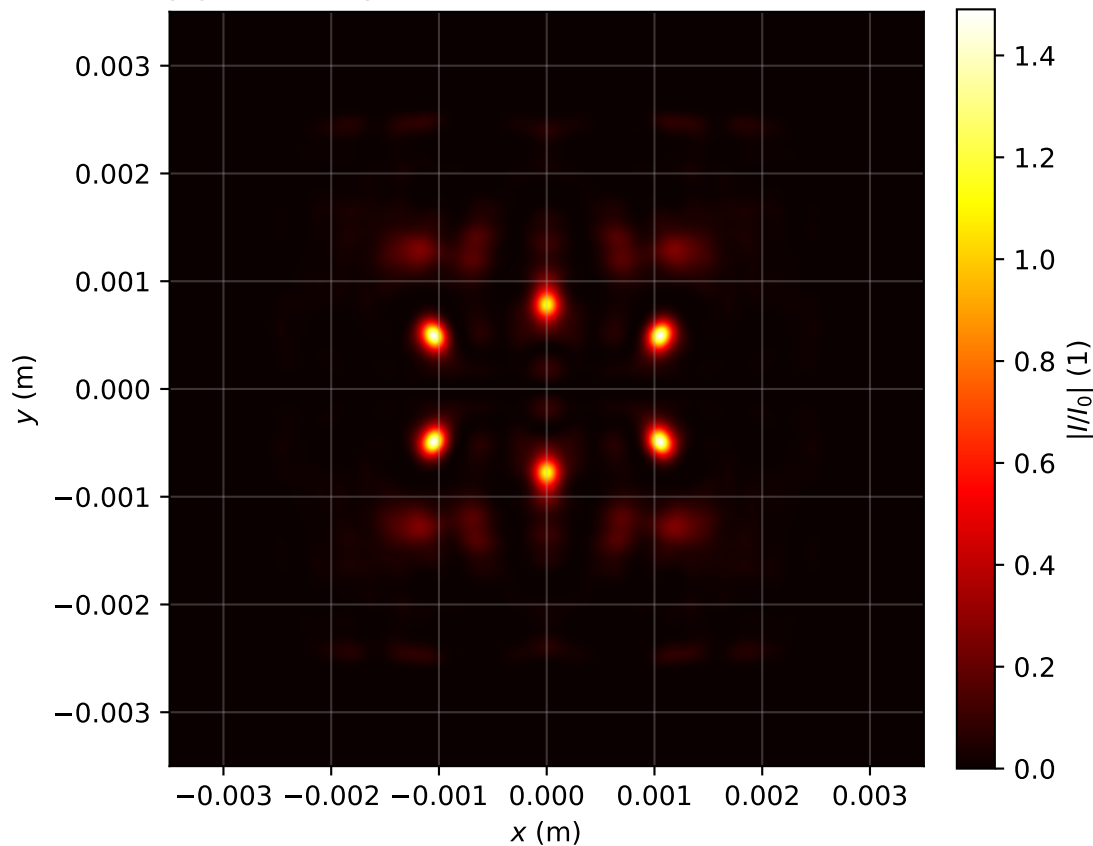
Intensity profile I(x, y, z = 2.229)/I_0 , P_{in}=20.0\text{Pcr} , artificial time
