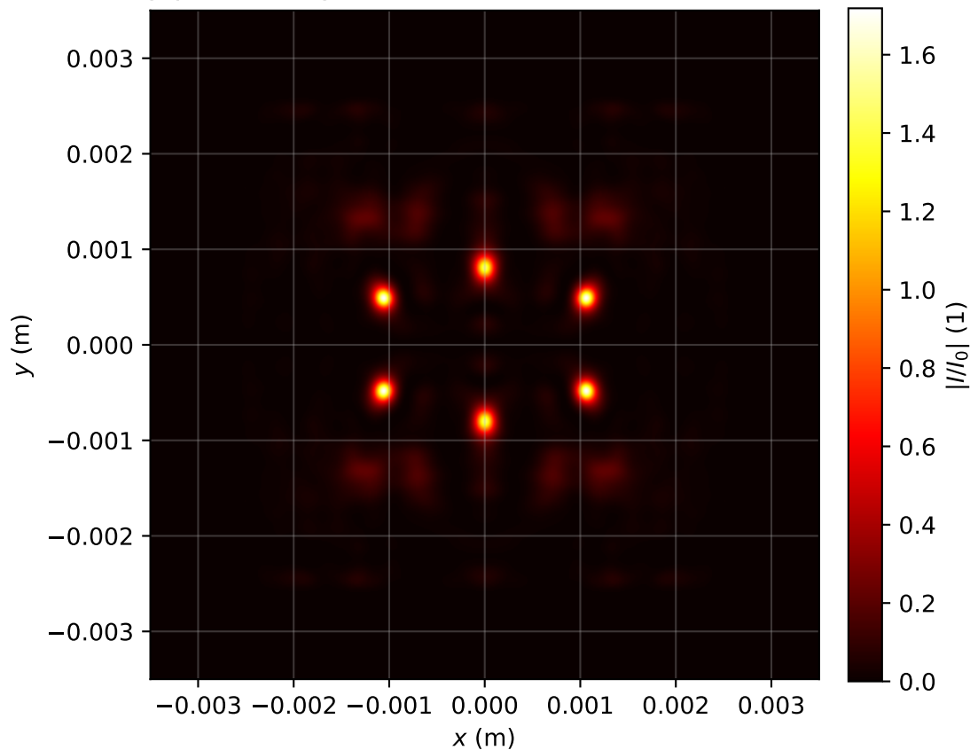
Intensity profile I(x, y, z = 2.309)/I_0 , P_{in}=20.0\text{Pcr} , artificial time
