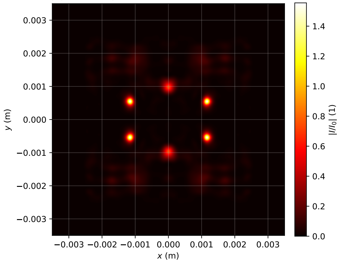
Intensity profile I(x, y, z = 2.866)/I_0 , P_{in}=20.0P_{cr} , artificial time
