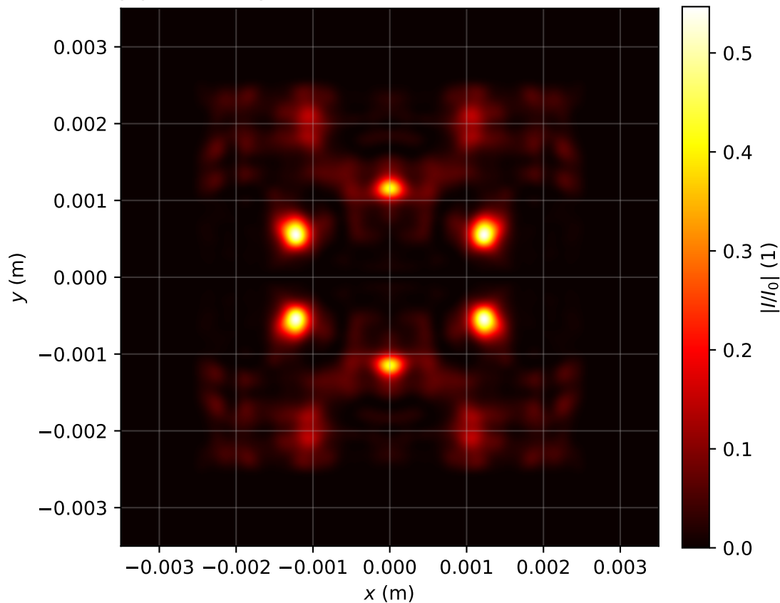
Intensity profile I(x, y, z = 3.184)/I_0 , P_{in}=20.0\text{Pcr} , artificial time
